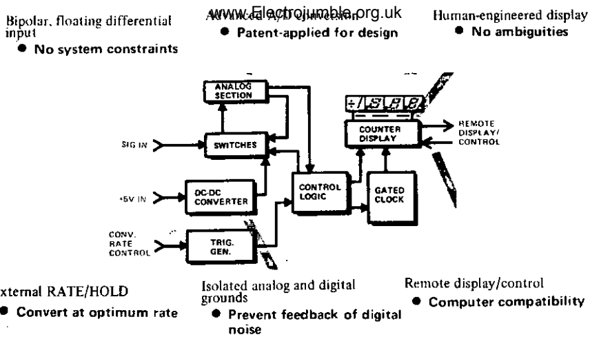
Figure 1. AN2535 Simplified Block Diagram.
